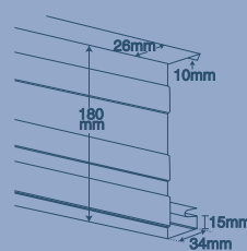
STEEL FASCIA
